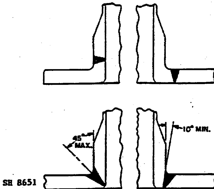
FIGURE 1. Examples of acceptable weld joint locations.
