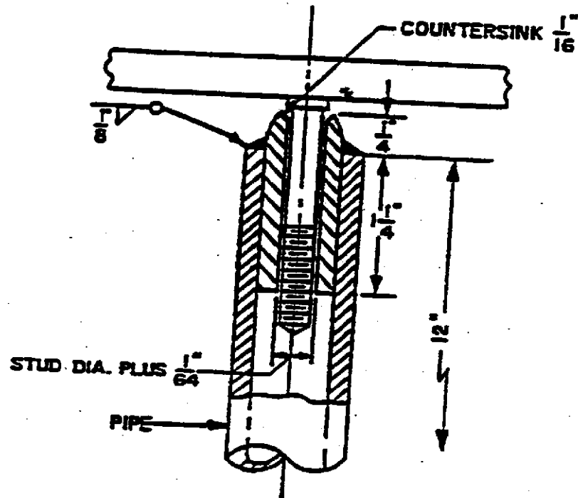
FIGURE 3. Device for testing welded studs.
