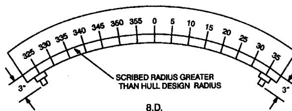
FIGURE 8. PARTIAL CIRCULARITY MEASUREMENTS. (see 5.5.1.a)
