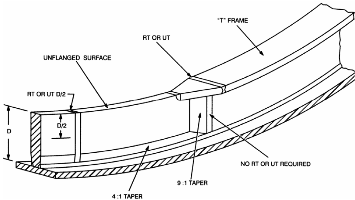
FIGURE 15. RT/UT REQUIREMENT FOR FLANGED TO UNFLANGED FRAME TRANSITIONS. (see Table 6-4, Cat 1.B(3))
