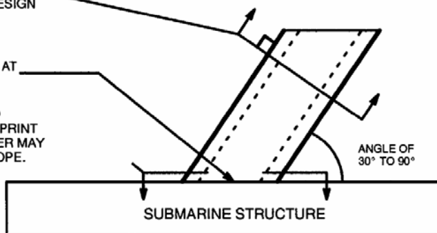
FIGURE 3. EXAMPLES OF MEMBERS FOR ATTACHMENT WELDS. (see 3.39.1)
