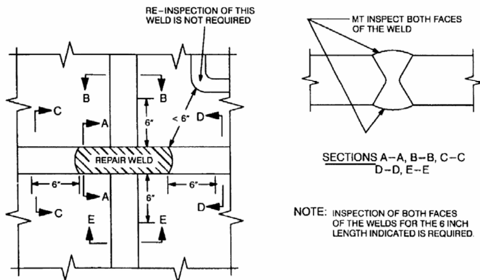
FIGURE 13. MT INSPECTION REQUIREMENTS FOR REPAIR OF FULL PENETRATION WELDS IN THE PRESSURE HULL ENVELOPE WHERE THE TOTAL REPAIR DEPTH IS GREATER THAN 1/3 T BUT LESS THAN OR EQUAL TO 2/3 T.
