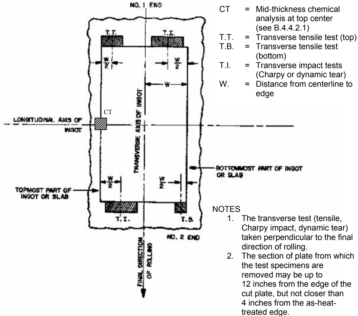
Figure B-4. Method of Locating Test Specimens for Conformance Inspection for Plates as Rolled Directly from Ingots or Slabs with the Final Direction of Rolling Parallel to the Transverse Axis of the Ingot.
